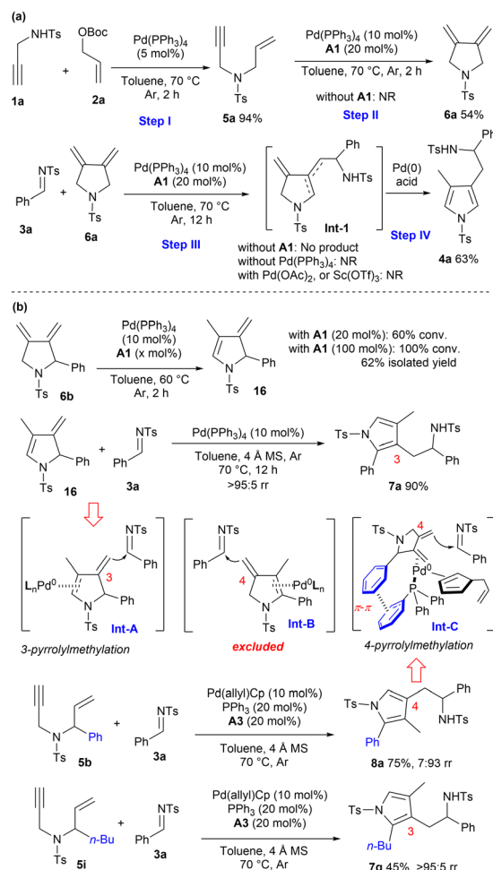
Scheme 5 Control experiments for mechanism and regioselectivity elucidation. (a) Elucidation of auto-tandem catalytic reaction. (b) Proposal of regiodivergent pyrrolylmethylation.
