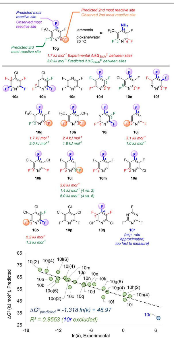
Fig. 10 Site selectivity predictions and rate correlation for S_NAr between fluorinated heterocycles and ammonia. Experimental data from ref. 99, 101, and 102.
