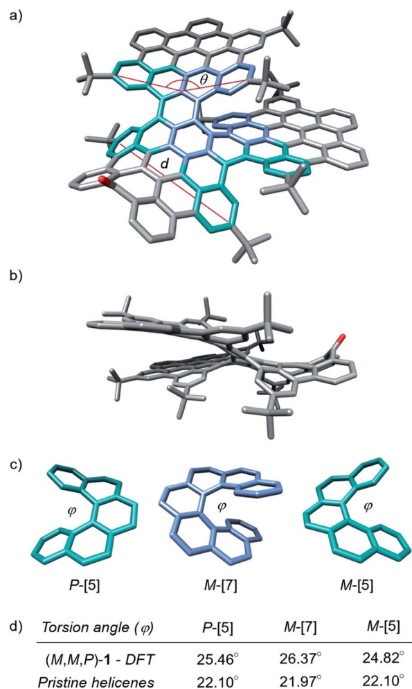
Fig. 2 (a) DFT optimized geometry of ( M,M,P )- 1 (CAM-B3LYP/6-31G(d,p), gas phase; lateral t Bu groups removed to reduce computational time); (b) side view; (c) [ n ]helicene structures extracted from the optimized geometry; (d) values of the measured torsion angles from the DFT optimized ( M,M,P )- 1 and XRD structures of pristine helicenes.
