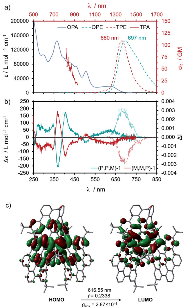
Fig. 3 (a) Experimental OPA (gray), OPE (turquoise, dashed), TPA (red) and TPE (red, dotted) spectra of (M,M,P/P,P,M) -1. Measured in \text{CHCl}_3 at ca. 1 \times 10^{-6} M, \lambda_{\text{exc}} = 370 nm for OPE, \lambda_{\text{exc}} = 900 nm for TPE; (b) experimental ECD spectra of (M,M,P) -1 (red) and (P,P,M) -1 (turquoise) measured in \text{CHCl}_3 at ca. 1 \times 10^{-6} M, and experimental CPL spectra ( \lambda_{\text{exc}} = 370 nm) of (M,M,P) -1 (pale red, dashed) and (P,P,M) -1 (pale turquoise, dashed) measured in \text{CHCl}_3 at ca. 1 \times 10^{-6} M; (c) HOMO and LUMO orbitals, and information of the TD-DFT calculated (CAM-B3LYP/6-31G(d,p)) lowest energy transition. The OPE spectrum is cropped at long wavelengths due to the use of a short path filter to block the multiphoton laser at the entrance of the photodetector.
