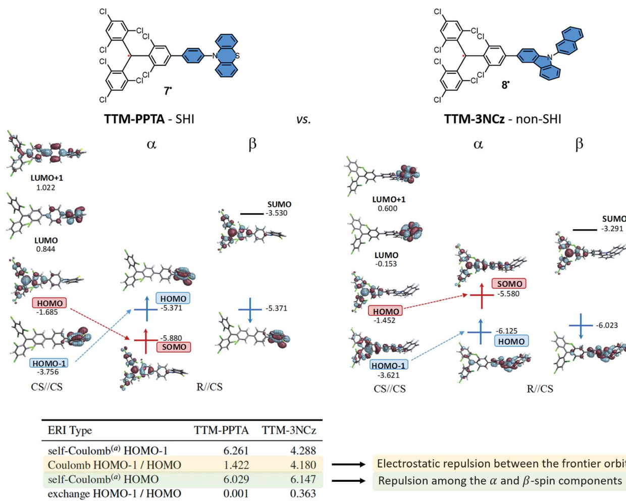
Fig. 6 Orbital energies (in eV) and isosurfaces (0.030 a.u.) of selected MOs of the TTM-PPTA, 7 and TTM-3NCz, 8 systems. See the text for a description of the CS//CS and R//CS labelling. The vertical dimension of the figure is associated with the orbital energy; however, as in other figures herein, the energy scales are drawn qualitatively and are not aligned. The table provides selected Coulomb and exchange electron repulsion integrals (ERIs, in eV) for the corresponding closed-shell parent systems. a Coulomb repulsion between the \alpha - and \beta -spin component of the MO. Figures adapted with permission from ref. 53. Copyright 2021 American Chemical Society.
