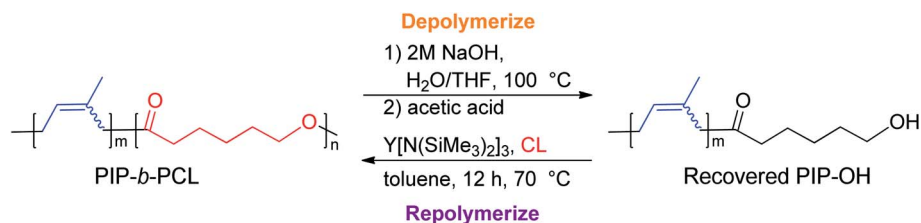
Fig. 5 Proposed selective hydrolysis of CL block and repolymerization to IP : CL diblock copolymer.
