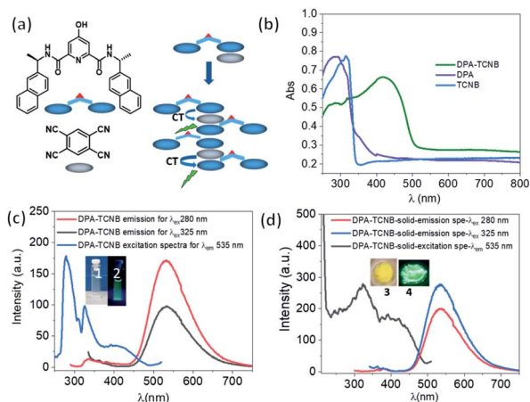
Fig. 3 (a) Schematic for charge transfer complex formation from the DPA and TCNB co-assembly; (b) solid-state absorption spectra of only DPA, TCNB and DPA-TCNB CT co-assembled materials, respectively; (c) emission spectra for \lambda_{\text{ex}} of 280 nm and 325 nm and excitation spectrum for \lambda_{\text{em}} of 535 nm for the DPA-TCNB suspension (~162 \mu\text{M} ); inset pictures 1 and 2: DPA-TCNB CT suspension in daylight and under a 365 nm UV lamp, respectively; (d) solid-state emission spectra of DPA-TCNB for \lambda_{\text{ex}} of 280 nm and 325 nm, respectively, and excitation spectrum for \lambda_{\text{em}} of 535 nm; inset pictures 3 and 4: DPA-TCNB CT powder in daylight and under 365 nm UV light, respectively.
