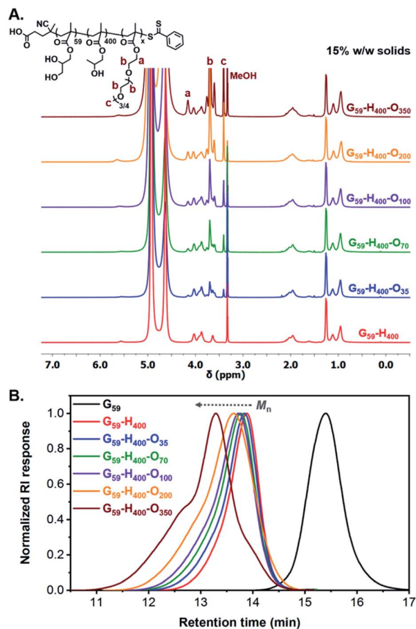
Fig. 2 (A) Stacked ^1\text{H} NMR spectra (CD _3 OD) recorded for a series of molecularly-dissolved \text{G}_{59}\text{-H}_{400}\text{-O}_x triblock copolymers (where x = 35, 70, 100, 200 or 350 ) prepared via RAFT-mediated aqueous PIDA at 15% w/w solids. (B) Normalized SEC traces (refractive index detector) recorded for the \text{G}_{59} precursor (black line), the \text{G}_{59}\text{-H}_{400} diblock copolymer (red line) and a series of \text{G}_{59}\text{-H}_{400}\text{-O}_x triblock copolymers (where x = 35 , blue line; x = 70 , green line; x = 100 , purple line; x = 200 , orange line; x = 350 , burgundy line) at 15% w/w solids (DMF + 10 mM LiBr eluent).
