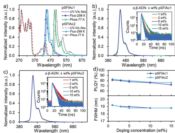
Fig. 2 (a) The absorption (left axis), fluorescence (right axis) spectra of pSFIAC1 and pSFIAC2 in toluene ( 10^{-5} \text{ M} ). (b) and (c) The PL spectra and transient PL (inset) curves with different concentrations in \alpha,\beta -ADN: x wt% MR emitters ( x = 1, 3, 5, 10, 15). (d) The PLQYs and FWHMs of the doped films with different concentrations in \alpha,\beta -ADN: x wt% MR emitters ( x = 1, 3, 5, 10, 15).
