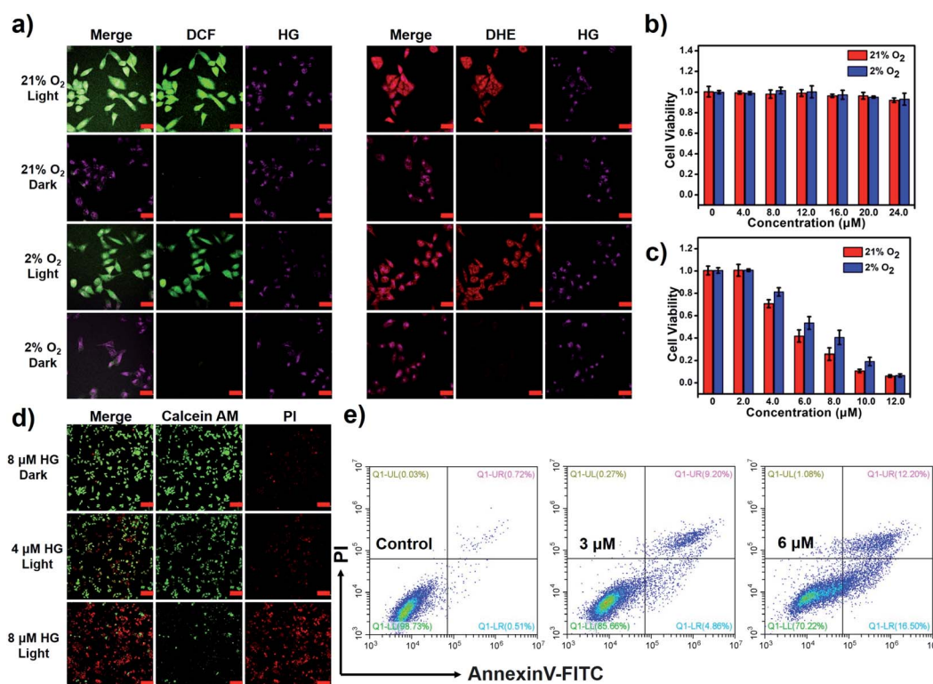
Fig. 5 (a) Detection of ROS and O 2 •− in HeLa cells with DCFH-DA and DHE under normoxia (21% O 2 ) or hypoxia (2% O 2 ) conditions. The scale bar represents 50 \mu m. Cell viability of HeLa cells subjected to a range of HG concentrations in the (b) absence and (c) presence of light-irradiation (660 nm, 50 mW cm −2 ) under normoxia or hypoxia conditions. (d) CLSM images of calcein AM/PI-stained HeLa cells. The scale bar represents 200 \mu m. (e) Apoptosis analysis of HeLa cells treated with HG at various doses (the parameter of CLSM: green channel: 500–550 nm, excited at 487 nm; red channel: 570–620 nm, excited at 562 nm; NIR channel: 663–738 nm, excited at 638 nm).
