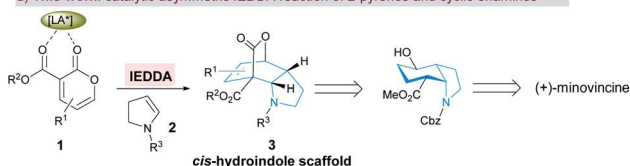
Scheme 1 Enantioselective synthesis of the cis -hydroindole scaffold.
