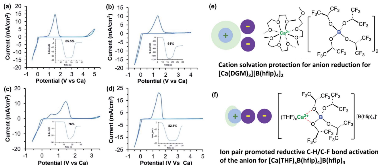
Fig. 11 Cyclic voltammograms of a 0.25 M \text{Ca}[\text{B}(\text{hfp})_4]_2 -DGM electrolyte solution with different working electrodes. (a) Glassy carbon working electrode. (b) Al working electrode with the inset showing accumulation of charge and coulombic efficiency. (c) Cu working electrode with the inset showing coulombic efficiency. (d) Pt working electrode with the inset showing coulombic efficiency. All samples were cycled at 100 \text{ mV s}^{-1} scan rate. (e) Proposed structure of \text{Ca}[\text{B}(\text{hfp})_4]_2 -DGM where \text{Ca}^{2+} and [\text{B}(\text{hfp})_4]^- are fully dissociated. (f) Proposed structure of partly solvated \text{Ca}[\text{B}(\text{hfp})_4]_2 -THF electrolyte where \text{Ca}^{2+} and [\text{B}(\text{hfp})_4]^- form an ion pair. Adapted with permission from ref. 40. Copyright 2020 Wiley-VCH.
