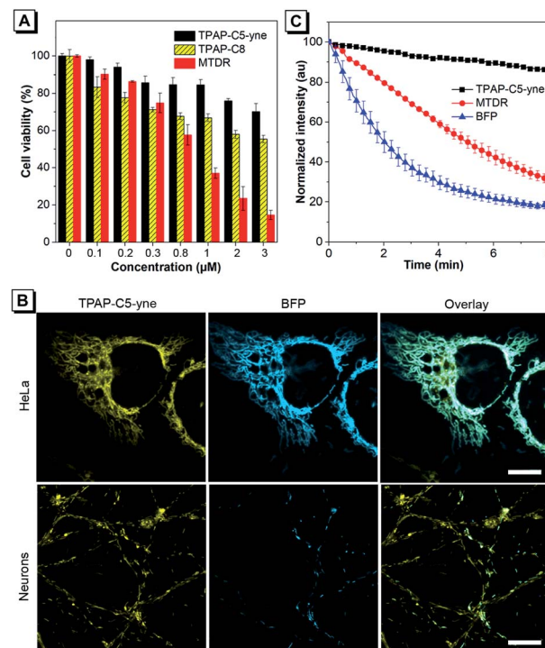
Fig. 3 (A) Cell viability of neurons stained with TPAP-C5-yne, TPAP-C8 and MTDR. (B) Co-localized images of HeLa cells and neurons stained with TPAP-C5-yne (300 nM) and Mito-BFP respectively. Scale bar: 10 \mu m. (C) Photostability of TPAP-C5-yne, MTDR, and BFP under continuous irradiation.
