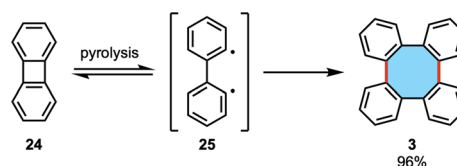
Scheme 10 Pyrolysis of biphenylene leading the synthesis of 3 .
