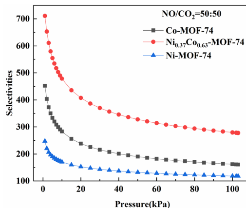
Fig. 6 Adsorption selectivity of \text{Co-MOF-74} , \text{Ni-MOF-74} and \text{Ni}_{0.37}\text{Co}_{0.63}\text{-MOF-74} for \text{NO}/\text{CO}_2 predicted by IAST model ( 298 \text{ K} ).
