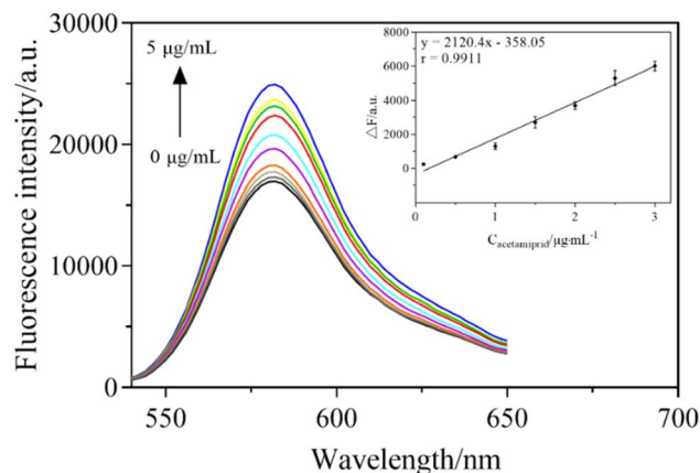
Fig. 9 Sensitivity of the fluorescent sensing system for acetamidrid detection. The fluorescence emission spectrum of the system in the presence of 0.1, 0.5, 1.0, 1.5, 2, 2.5, 3.0, 4.0, 5.0 \mu g mL^{-1} acetamidrid. Inset: the linear regression method was used to draw the experimental curve. The linear range of the sensing system for acetamidrid was 0.1–3 \mu g mL^{-1} . All measurements were performed at 25 °C with excitation at 510 nm.
