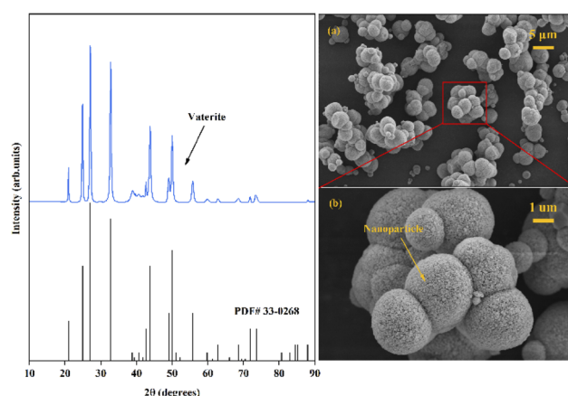
Fig. 5 XRD and SEM images ((a) scale bar 5 μm, (b) scale bar 1 μm) of the obtained \text{CaCO}_3 products.
