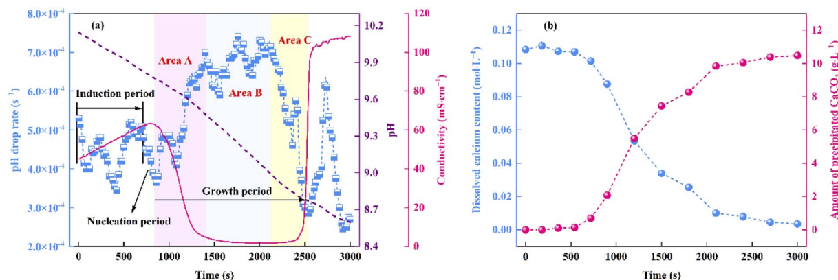
Fig. 3 Variations in the (a) pH and conductivity of the reaction system over time. (b) Contents of dissolved Ca and precipitated \text{CaCO}_3 during the progress of the carbonation reaction.
