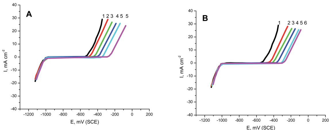
Fig. 5 PDAP curves of S-Fe corrosion in the free 1.0 M HCl + 0.5 M NaCl solution and when containing different concentrations of (A) PS and (B) PBT at 300 K at a scan rate of 0.2 mV s -1 : (1) 0.0, (2) 100, (3) 200, (4) 300, (5) 400, (6) 500 mg l -1 .
