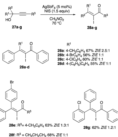
Scheme 18 Propargyl alcohols iodination with 5 mol% \text{AgSbF}_6 .
