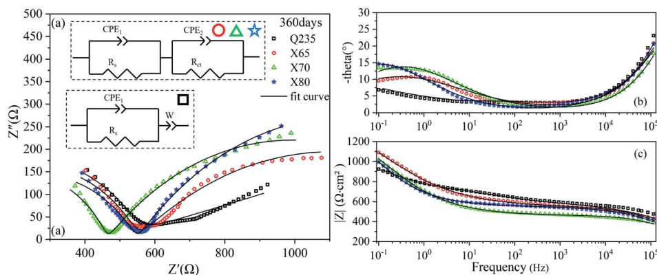
Fig. 8 EIS diagrams of Q235, X65, X70, and X80 steel samples after 360 days of corrosion: (a) Nyquist diagram; (b), (c) Bode diagrams.
