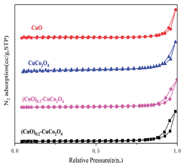
Fig. 5 \text{N}_2 adsorption-desorption isotherm curves of all samples.
