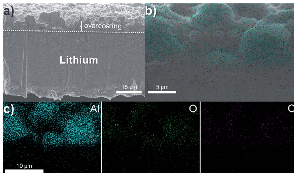
Fig. 3 (a) SEM image and (b, c) the corresponding elemental mapping in Al (blue), O (green) and C (purple) of a LiAl with an overcoating of 50% \text{Al}_2\text{O}_3 -ndl ( \sim 6\text{--}7\ \mu\text{m} ).
