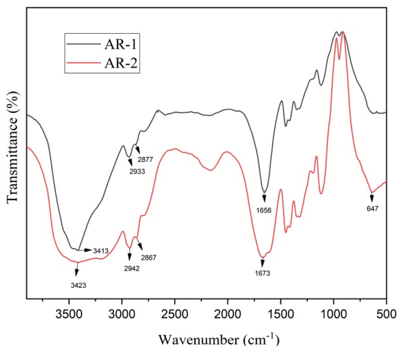
Fig. 1 The FT-IR spectra of AR-1 and AR-2.
