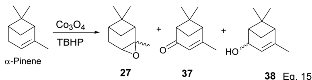
Scheme 12 Cobalt oxide-promoted transformation of \alpha -pinene.
