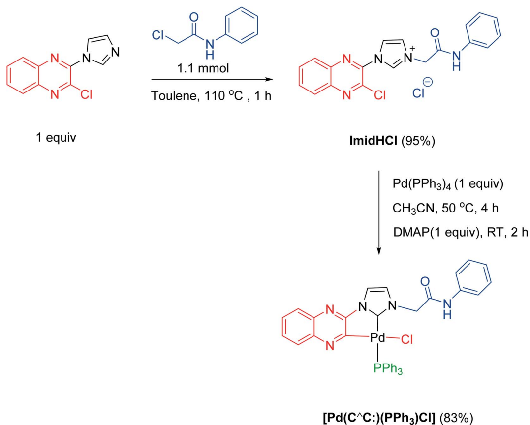
Scheme 2 Synthesis of palladacycle [\text{Pd}(\text{C}^{\text{A}}\text{C}:)(\text{PPh}_3)\text{Cl}] .
