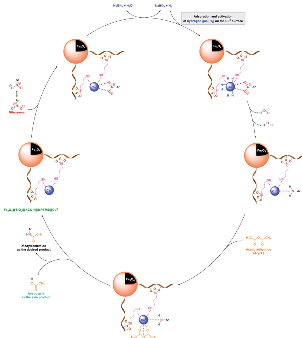
Scheme 2 Plausible mechanism of the one-pot reductive acetylation of nitroarenes catalyzed by the \text{Fe}_3\text{O}_4@ \text{SiO}_2@ \text{KCC-1}@ \text{MPTMS}@ \text{Cu}^{\text{II}} nanocomposite in water.
