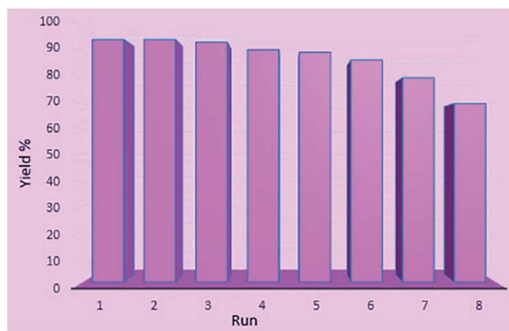
Fig. 6 Reusability of \text{Ni}^{\text{II}}(\text{BAPTE})(\text{NO}_3)_2\text{-Cell} nanocatalyst in the reaction of isatin (1 mmol), malononitrile (1 mmol) and dimesoxane (1 mmol).
