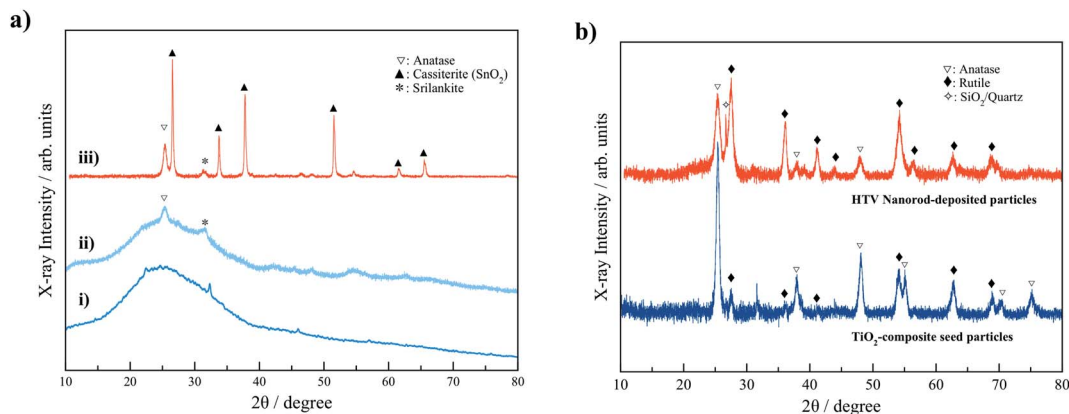
Fig. 7 (a) X-ray diffraction patterns of (i) \text{TiCl}_4 -treated seed particles, (ii) nanowire-deposited particles via CDB method and (iii) nanowires grown on FTO glass slides via CBD method. (b) X-ray diffraction patterns of the \text{TiO}_2 -composite seed particles and the nanorod-deposited particles via HTV method.
