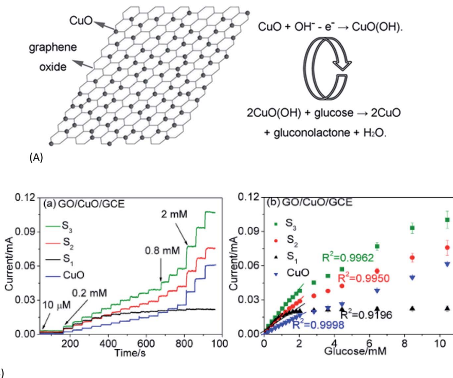
Fig. 6 (A) Illustration of the non-enzymatic glucose sensing mechanism using the CuO/GO composite. (B) Amperometric responses of GO–CuO electrodes with increasing CuO loading ( \text{S}_1 – \text{S}_3 ) to the successive addition of glucose [this figure has been reproduced from ref. 109 with permission from American Chemical Society, Copyright 2013].
