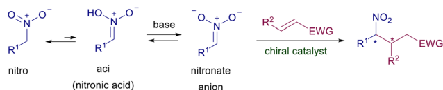
Scheme 1 Aci-nitro equilibrium and conjugate addition to electron-poor alkenes.
