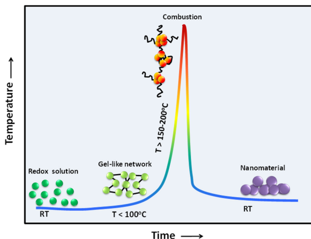
Fig. 8 Pictorial representation of the temperature and structure evolution of SCS-synthesized nanomaterials from the redox solution reaction to the formation of a redox network and subsequent combustion reaction. The combustion material would require an additional calcination step if residual carbon material needed to be removed.
