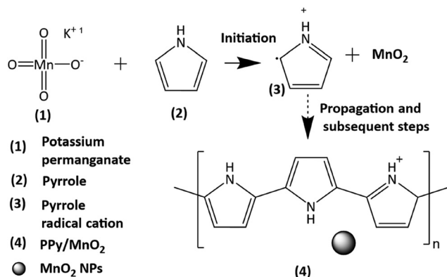
Scheme 1 The mechanism of the redox initiated polymerization of a pyrrole monomer in the presence of KMnO 4 as an oxidant to give PPy/MnO 2 . The mechanism involves the formation of a pyrrole radical cation in the initiation step and subsequently leads to the formation of PPy/MnO 2 with attached MnO 2 NPs.
