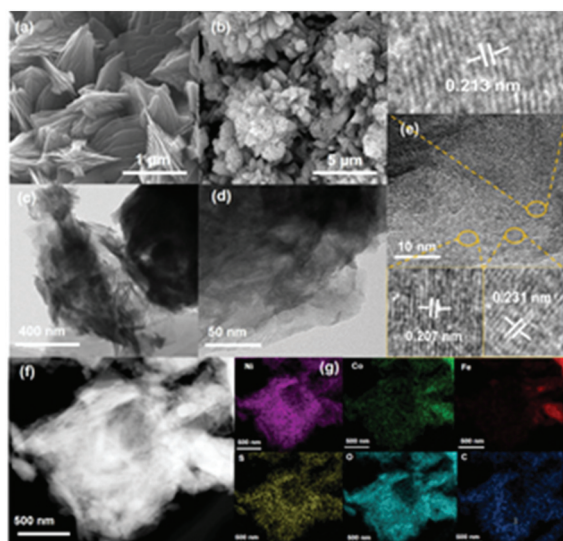
Fig. 1 (a) SEM morphologies of FeCoNi-NS. (b) SEM image, (c) and (d) TEM images, (e) HRTEM image, (f) and (g) HAADF-STEM image and the corresponding element mappings of Fe, Co, Ni, S, C, and O in FeCoNi-NS-ACVs.
