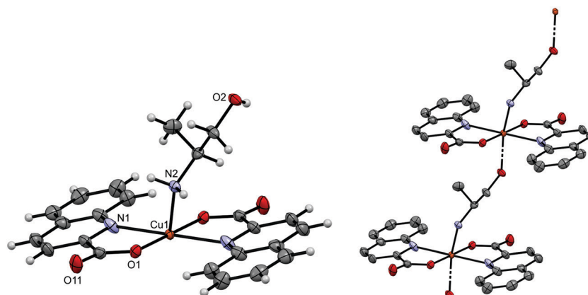
Fig. 3 ORTEP drawings of a repeating unit (left) and a short section of a chain (right) in [\text{Cu}(\text{quin})_2(2\text{a1pOH})]_n ( 8c ). The Cu(II) coordination sphere is completed by the O1, N1 and N2/O2 ( 1-x, 1-y, 1-z ) symmetry equivalents. Displacement ellipsoids are drawn at the 50% probability level. Hydrogen atoms are shown as spheres of arbitrary radii (left) or omitted for clarity (right).
