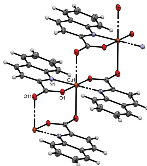
Fig. 8 ORTEP drawing of a short section of a chain in [Cu(quin) 2 ] n (g). Displacement ellipsoids are drawn at the 50% probability level. Hydrogen atoms are shown as spheres of arbitrary radii. The Cu(II) coordination sphere is completed by the O11 (−x, 1 − y, 1 − z and 1 + x, y, z), N1 and O1 (1 − x, 1 − y, 1 − z) symmetry equivalents. The Cu–N bond lengths are 2.0907(12) Å, and the Cu–O bond lengths are 1.9089(10) and 2.5772(12) Å.
