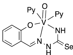
Fig. 10 Salicylaldehyde selenosemicarbazone as a dianionic [\text{O}, \text{N}, \text{N}]^{2-} ligand.
