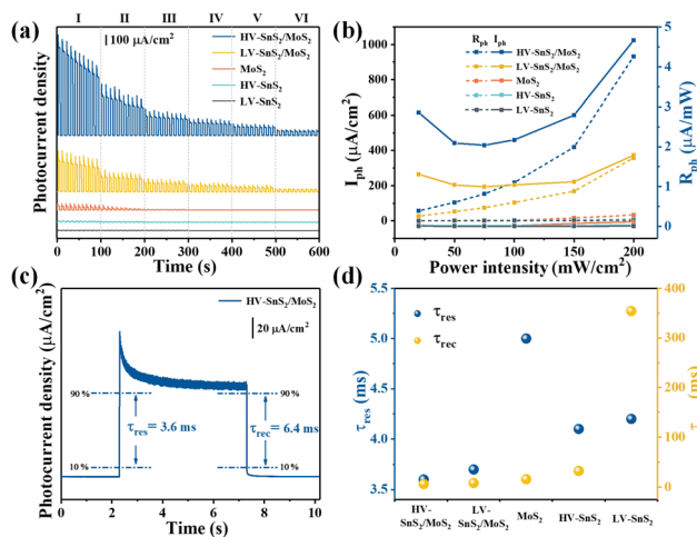
Fig. 5 Photoresponse performances of all samples as photoanodes in 1 M \text{Na}_2\text{SO}_4 under 0 V. (a) The amperometric I - t curves irradiated by different simulated solar light power intensities (From I to VI: 200, 150, 100, 75, 50, 20 \text{mW cm}^{-2} ). (b) Photocurrent density ( I_{\text{ph}} ) and photoresponsivity ( R_{\text{ph}} ) as a function of the light power intensity. (c) The time constants of HV-SnS 2 /MoS 2 for the response ( t_{\text{res}} ) and recovery ( t_{\text{rec}} ). (d) The t_{\text{res}} and t_{\text{rec}} of the samples.
