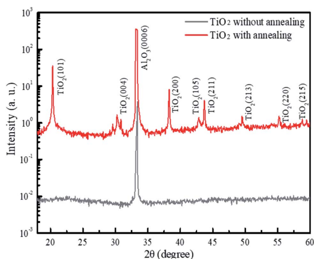
Fig. 3 XRD patterns of the \text{TiO}_2 film on the sapphire substrate with and without annealing at 450 °C for 3 h.
