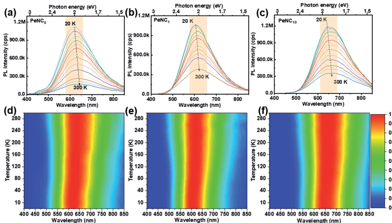
Fig. 4 Temperature-dependent PL spectra of (a) \text{PeNC}_0 ( \lambda_{\text{ex}} = 275 nm), (b) \text{PeNC}_1 ( \lambda_{\text{ex}} = 330 nm), and (c) \text{PeNC}_{10} ( \lambda_{\text{ex}} = 330 nm) from 20 to 300 K. Normalized PL intensity mapped with the emission wavelength and temperature for (d) \text{PeNC}_0 (e) \text{PeNC}_1 , and (f) \text{PeNC}_{10} .
