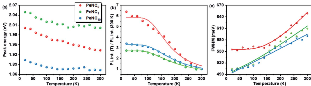
Fig. 5 Temperature-dependent PL (a) emission peak energy, (b) peak intensity, and (c) FWHM of \text{PeNC}_0 , \text{PeNC}_1 , and \text{PeNC}_{10} .
