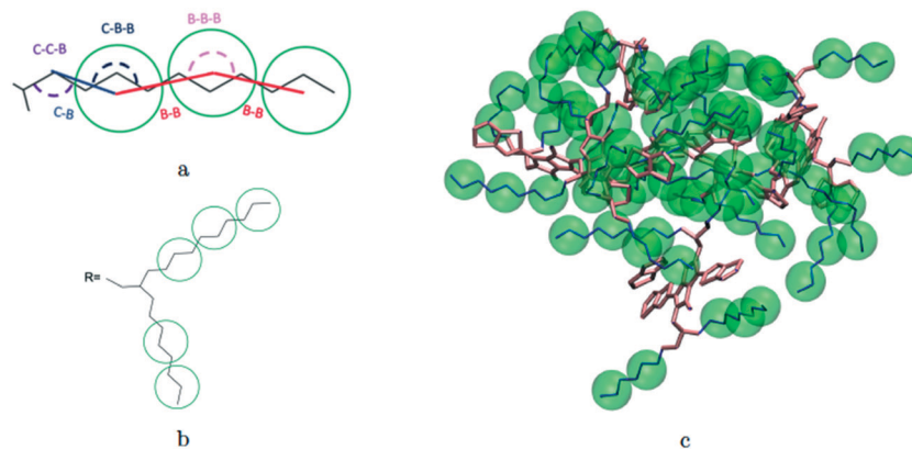
Fig. 2 Bead mapping schematic for TTT as an example system with atomic representations in lines and beads in green spheres. a) Extra bonded force-field parameters introduced for the hybrid model; b) bead mapping along a side chain; c) a sample snapshot. Hydrogens are omitted for simplicity.
