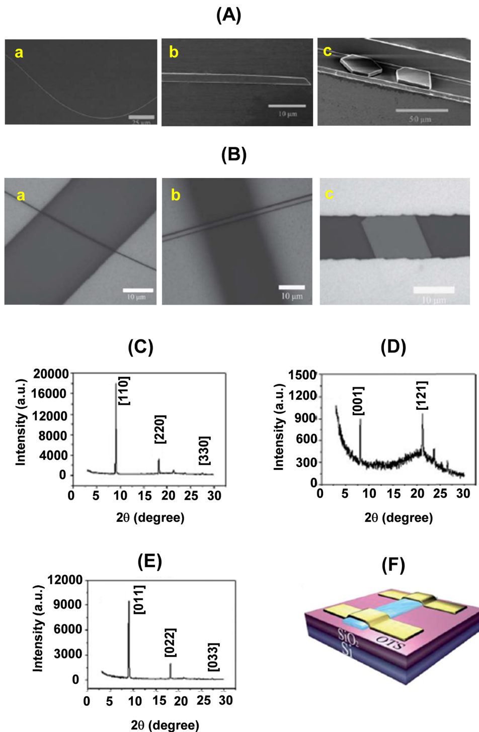
Fig. 11 (A) SEM images of an individual wire (a), ribbon (b) and plate (c) of 22a–c , respectively; (B) optical images (a, b and c) of the SCO-FET devices of 22a–c , respectively; (C–E) powder diffraction patterns of the wires, ribbons and plates of 22a–c , respectively. The peaks are indexed with lattice constants of the bulk crystals; (F) schematic structure of a BGTC SCO-FET device. Reproduced with permission from ref. 16. Copyright 2013, The Royal Society of Chemistry.
