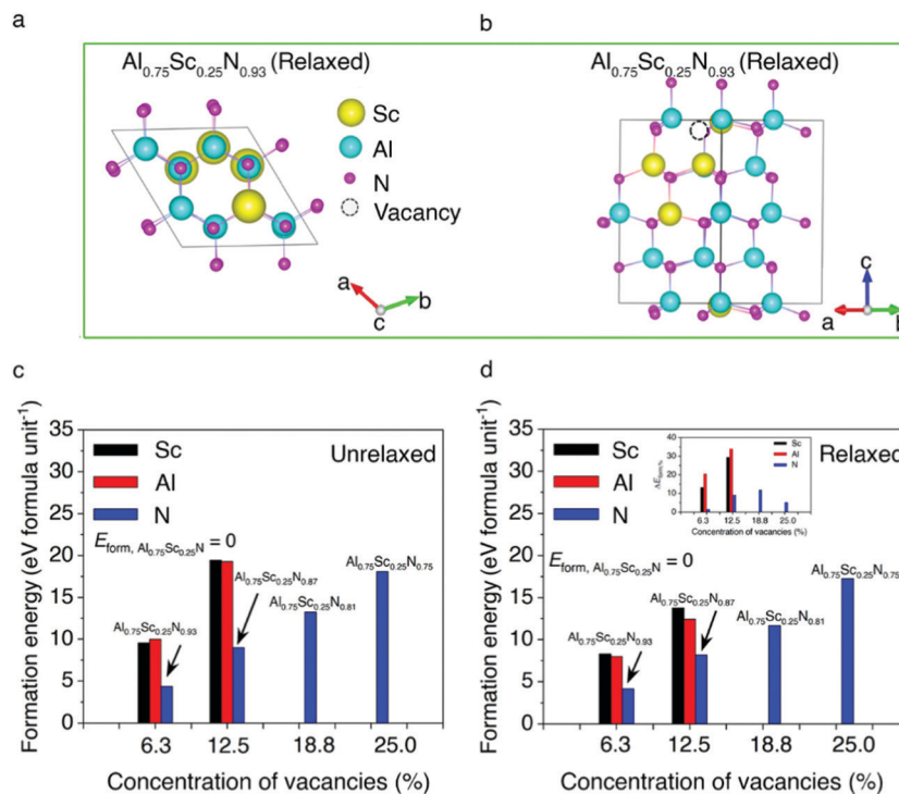
Fig. 1 Wurtzite structure and defect formation energies of the AlScN systems with vacancies. (a) Top and (b) side-view snapshots of the AlScN system. Sublattice A contains N atoms (magenta), and sublattice B comprises Sc atoms (yellow) and Al atoms (cyan). (c and d) Formation energies for different concentrations of Al, Sc and N vacancies for the (c) unrelaxed and (d) relaxed models. Inset in (d) shows the plot of percentage decrease in defect formation energy ( \Delta E_{\text{form},\%} = \frac{|E_{\text{form,relaxed}} - E_{\text{form,unrelaxed}}|}{E_{\text{form,unrelaxed}}} \times 100\% ) as a function of vacancy concentrations. There is no data for the models with Al and Sc vacancy concentrations between 18.8% and 25.0% because these models can show large structural changes.
