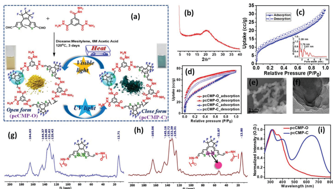
Fig. 21 (a) Preparation of the pcCMP (b) PXRD for pcCMP-O; (c) \text{N}_2 adsorption (77 K) for pcCMP-O; (d) \text{CO}_2 adsorption for pcCMP-O and pcCMP-C; (e) FESEM and (f) TEM images for pcCMP-O; (g and h) solid-state ^{13}\text{C} NMR for pcCMP-O and pcCMP-C, respectively; and (i) UV-vis absorption spectra in the solid state for pcCMP-O and pcCMP-C. Reproduced from ref. 152 with permission from American Chemical Society.
