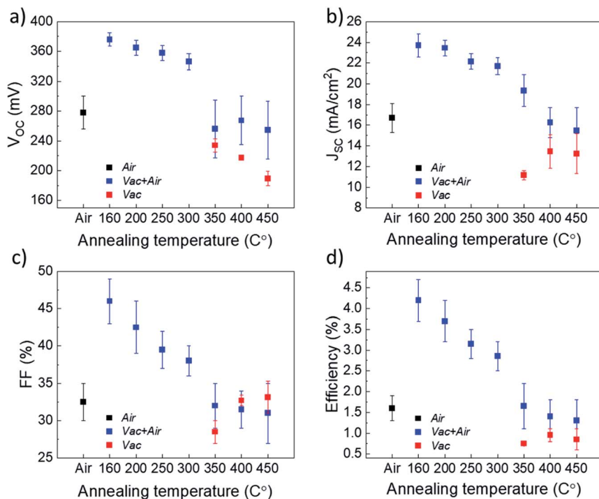
Fig. 3 J–V parameters, including (a) open-circuit voltage – V_{OC} , (b) short-circuit current density – J_{SC} , (c) fill factor – FF and (d) efficiency of TiO 2 /Sb 2 Se 3 devices with different TiO 2 annealing conditions.
