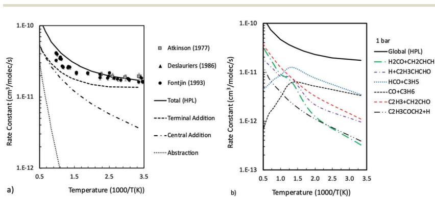
Fig. 4 Total rate constants for the \text{O}(^3\text{P}) + 1,3\text{-butadiene} reaction compared with experimental data 48,50,51 and contributions of addition to central and terminal carbon atoms and abstraction (a), and channel specific rate constants computed as a function of temperature at 1 bar (b).
