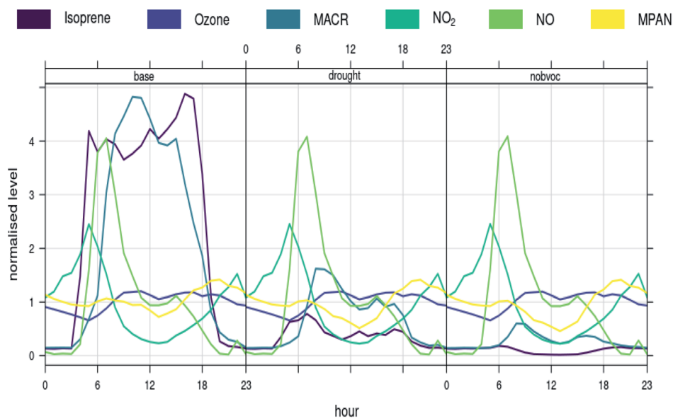
Fig. 8 Normalized mean diurnal variations for MACR, MPAN, isoprene, ozone, NO and NO 2 in July for different scenarios at HP. Time in hours on the x-axis refers to local time.
