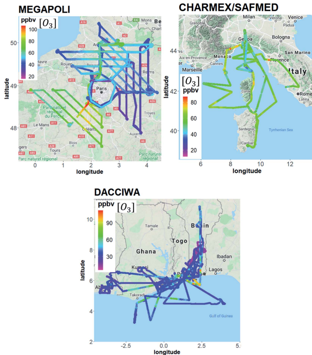
Fig. 2 MEGAPOLI, ChArMEx/SAFMED and DACCWA aircraft flights color-coded by ozone mixing ratios in ppbv.
