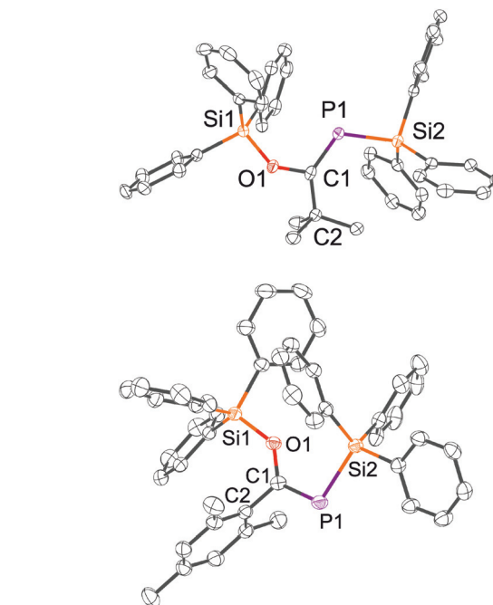
Fig. 1 Structure of E -10 (top) and Z -11 (bottom) in the crystal (hydrogens omitted for clarity). Selected bond distances [Å] and angles [ ^\circ ] for E -10: Si1–O1 1.6871(17); O1–C1 1.354(3); P1–C1 1.704(2); Si2–P1 2.2604(9); C1–C2 1.497(3); C2–C1–P1 117.33(17); O1–C1–P1 124.47(18); C1–P1–Si2 102.34(9); Si2–P1–C1–O1 6.1(2); P1–C1–O1–Si1 12.73(13); for Z -11: Si1–O1 1.6688(19); O1–C1 1.372(3); P1–C1 1.718(3); Si2–P1 2.2696(10); C1–C2 1.528(4); C2–C1–P1 137.92(19); O1–C1–P1 114.02(19); O1–C1–C2 108.1(2); C1–P1–Si2 113.82(9); Si2–P1–C1–O1 12.58(15); P1–C1–O1–Si1 37.6(3).
