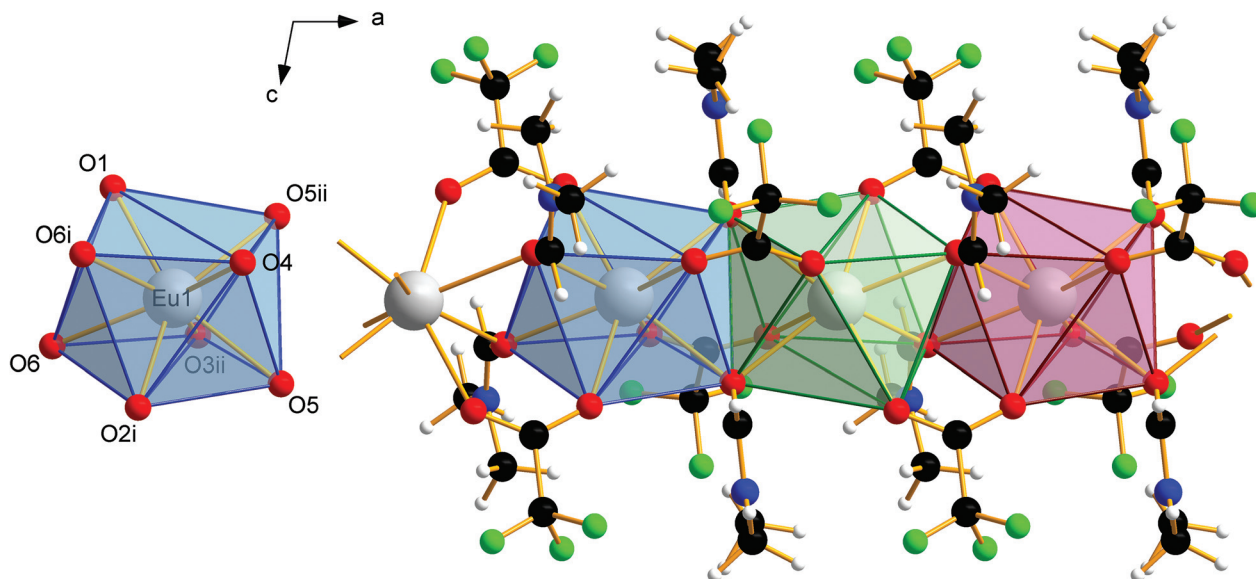
Fig. 3 Coordination polyhedron of Eu1 in 1 (left). Symmetry codes: (i) 1-x, 1-y, 1-z ; (ii) -x, 1-y, 1-z . Note the eightfold coordination of the \text{Eu}^{2+} ions by oxygen atoms in square antiprismatic coordination polyhedra. Section of the coordination polymer 1 , with four repeating units (right). Direction of view against the crystallographic b -axis. The \text{Eu}^{2+} ions are linked by two bridging trifluoroacetato ligands and two bridging molecules of N,N -dimethylformamide. The individual coordination polyhedra are edge-linked to each other. Color code: C (black), H (white), N (blue), O (red), F (green), Eu (gray).
