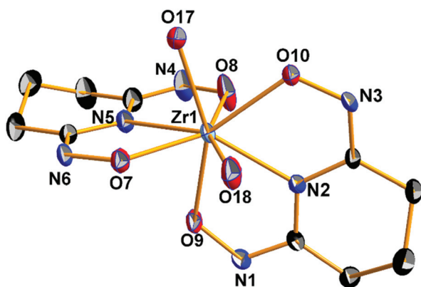
Fig. 1 ORTEP plot (50% probability level) of the cation [\text{Zr}^{\text{IV}}(\eta^1, \eta^1, \eta^1\text{-H}_2\text{pidiox-O,N,O}')_2(\text{OH})_2]^{2+} of 1 with a partial labeling scheme.
