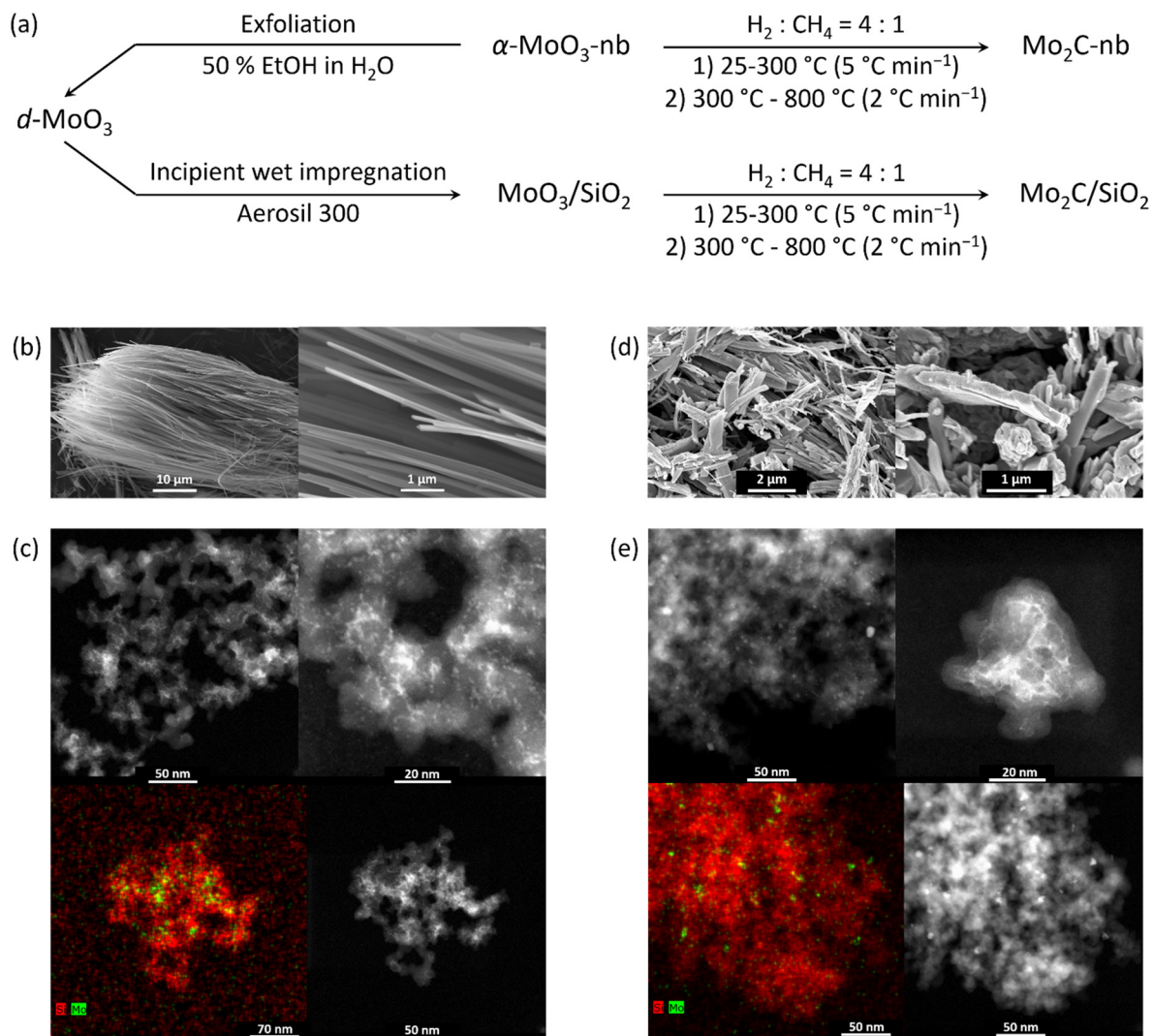
Fig. 1 a) Synthesis of Mo 2 C-nb from \alpha -MoO 3 -nb and Mo 2 C/SiO 2 from silica-supported delaminated MoO 3 films MoO 3 /SiO 2 ; b) SEM images of as synthesized \alpha -MoO 3 -nb; c) HAADF-STEM images and EDX elemental (Si and Mo) maps of MoO 3 /SiO 2 ; d) SEM images of Mo 2 C-nb; and e) HAADF-STEM images and EDX maps of Mo 2 C/SiO 2 .
