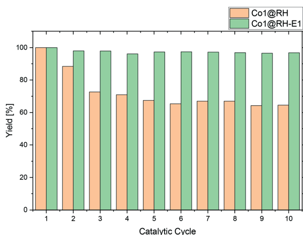
Fig. 8 Catalyst recycling test over 10 runs using un-etched (Co1@RH) and etched (Co1@RH-E1) catalysts. Reaction conditions: 120 °C, 10 bar H 2 , 200 mg of catalyst, nitrobenzene (8 mmol), isopropanol (0.5 ml) and water (0.5 ml).
